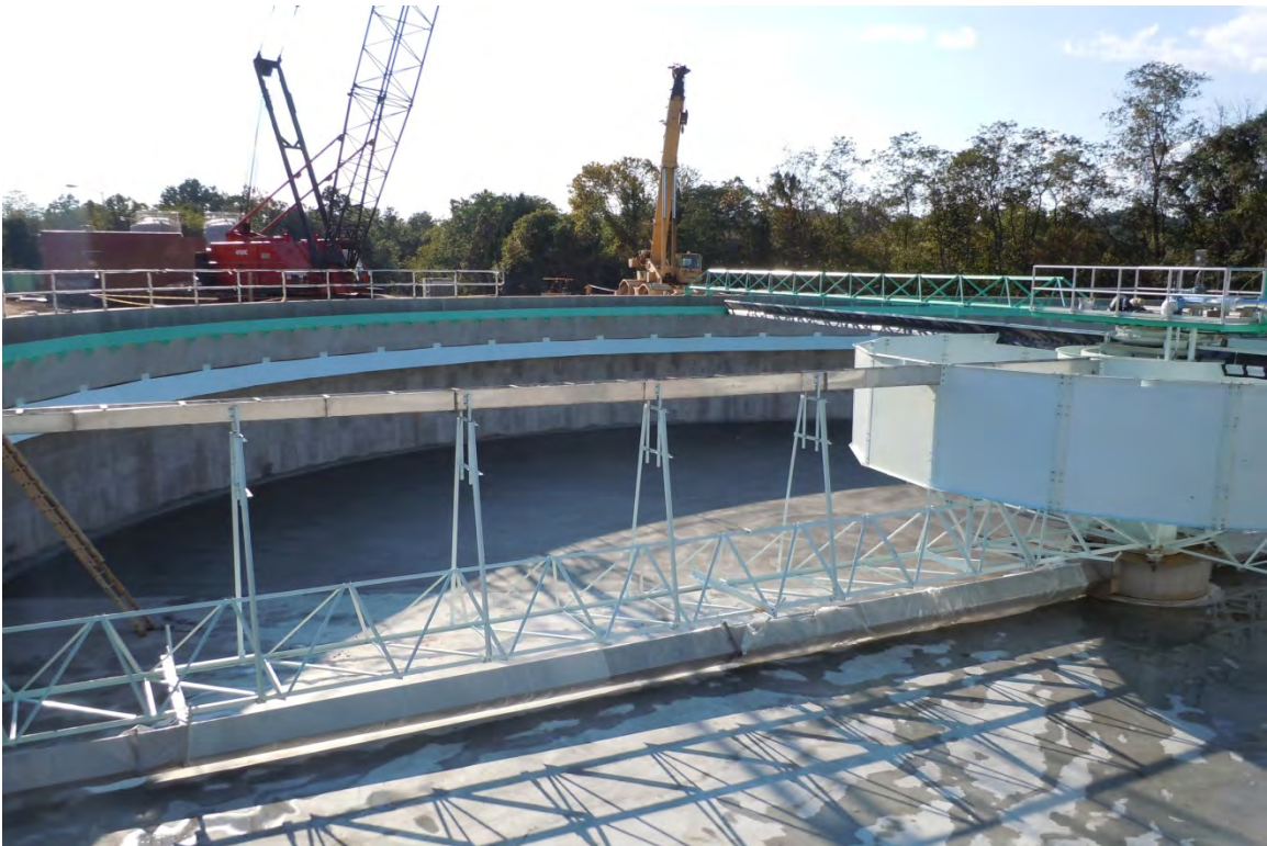
Interior of Secondary Clarifier No. 3
